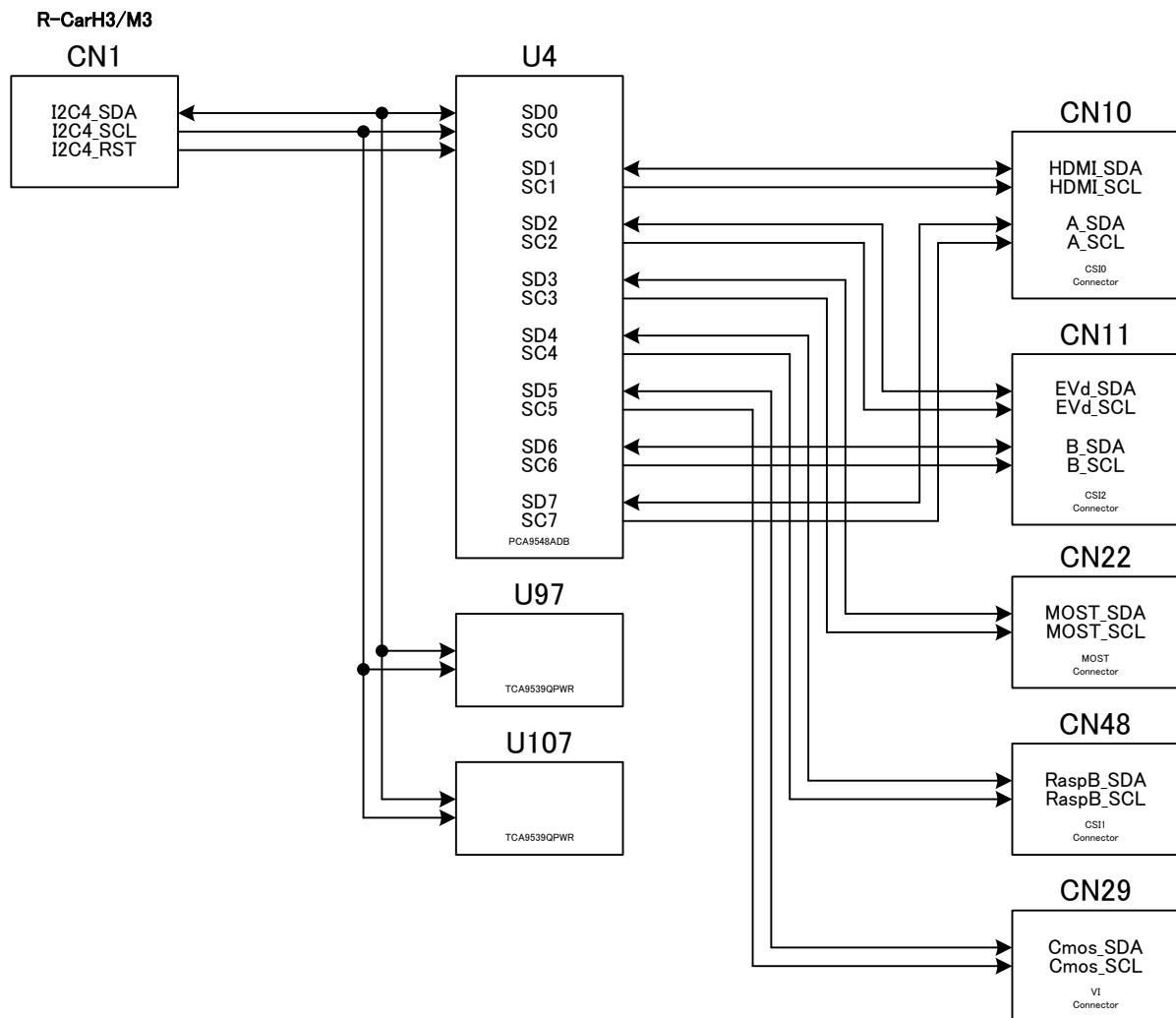
Figure 4-23b : I2C I/F
