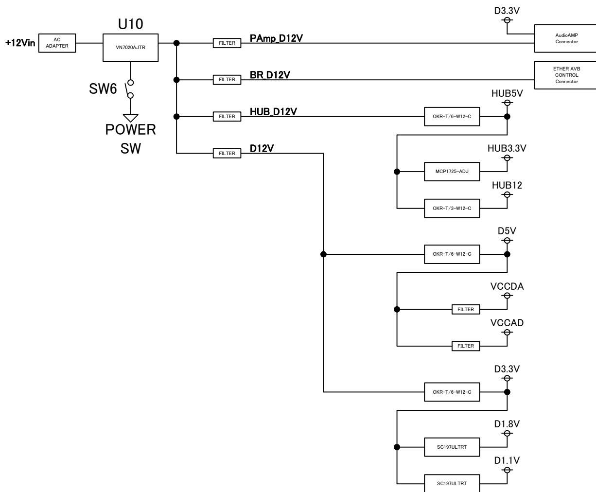
Figure 4-1 : Power structure
