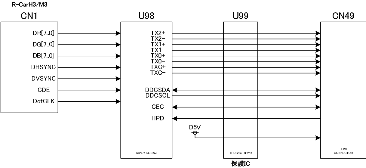
Figure 4-13 HDMI I/F
