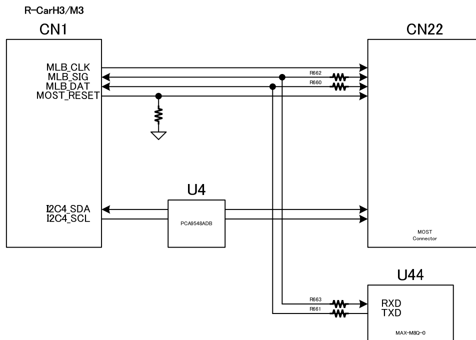
Figure 4-18 : MOST I/F
