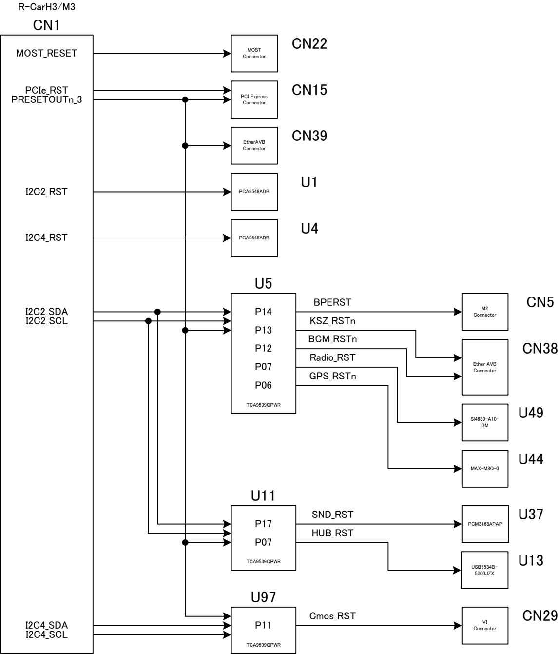
Figure 4-2 : Reset structure
