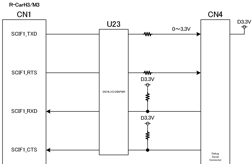
Figure 4-10 : SERIAL I/F
