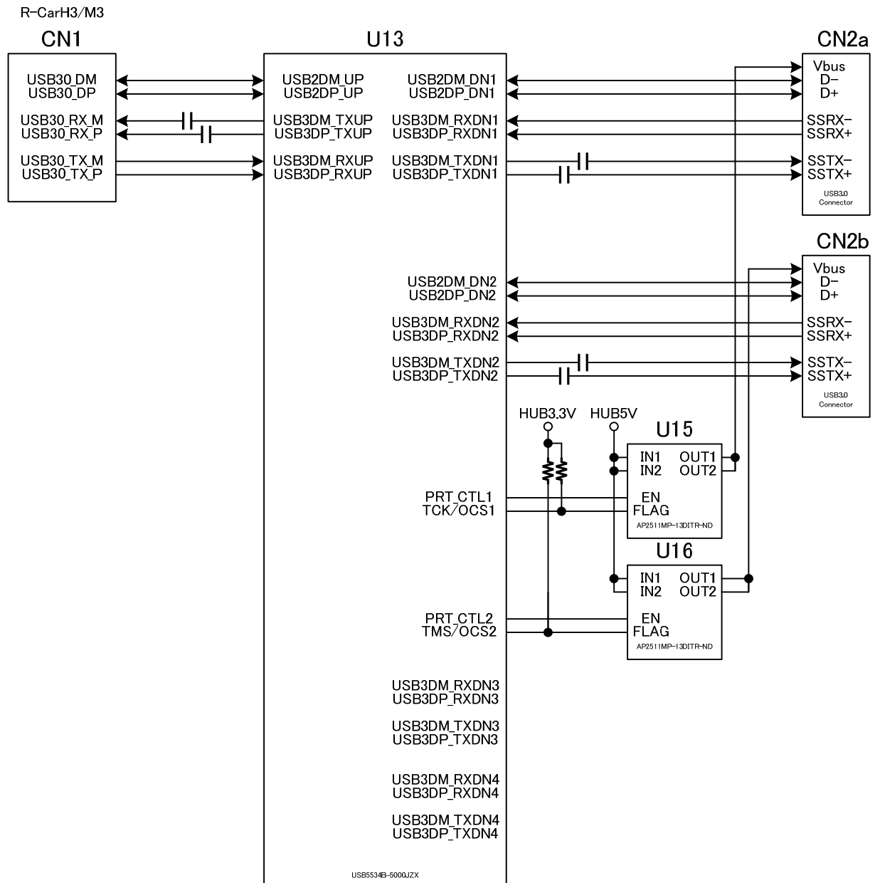
Figure 4-4 : USB 3.0 I/F
