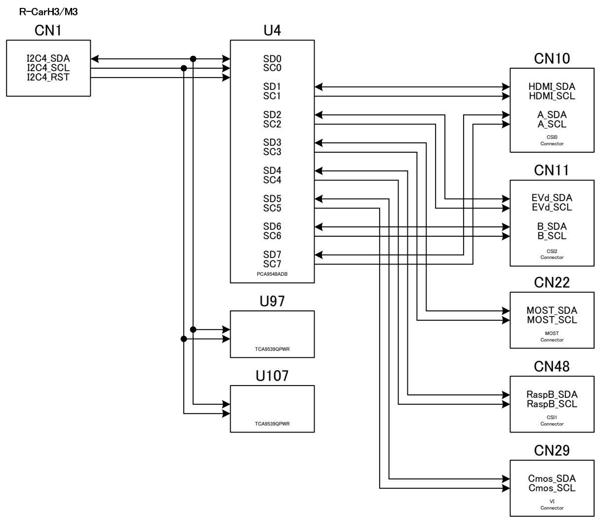
Figure 4-23b : I2C I/F
