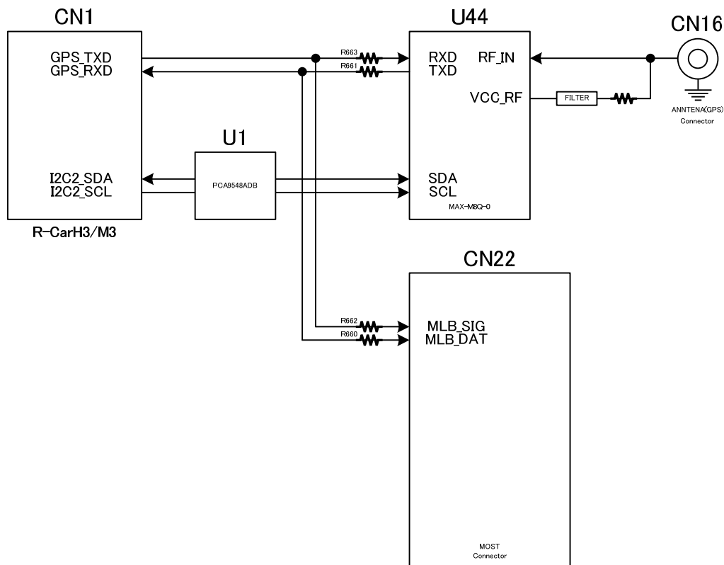
Figure 4-19: GPS I/F
