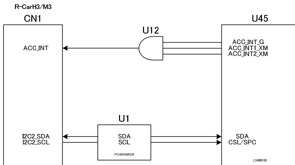
Figure 4-21 : 9 axis sensor I/F
