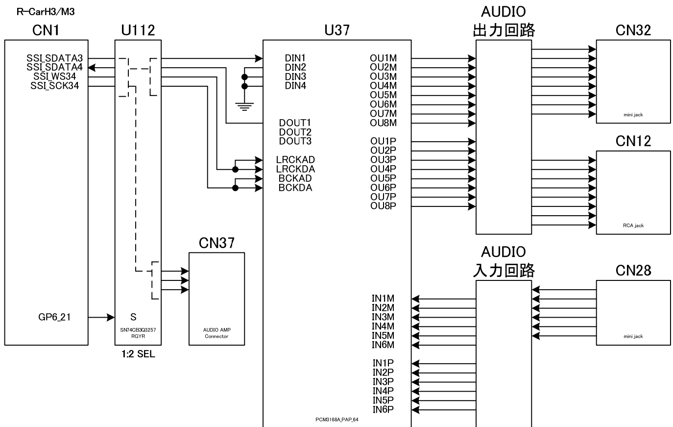
Figure 4-15 AUDIO I/F
