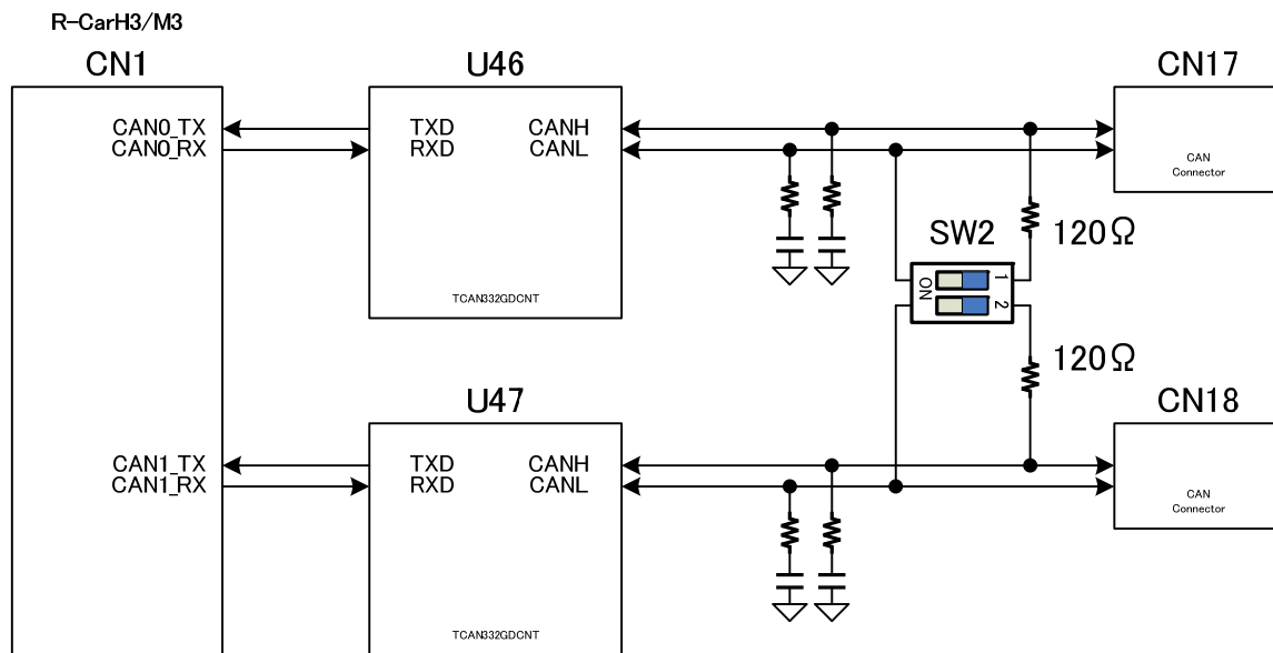
Figure 4-17 CAN I/F
